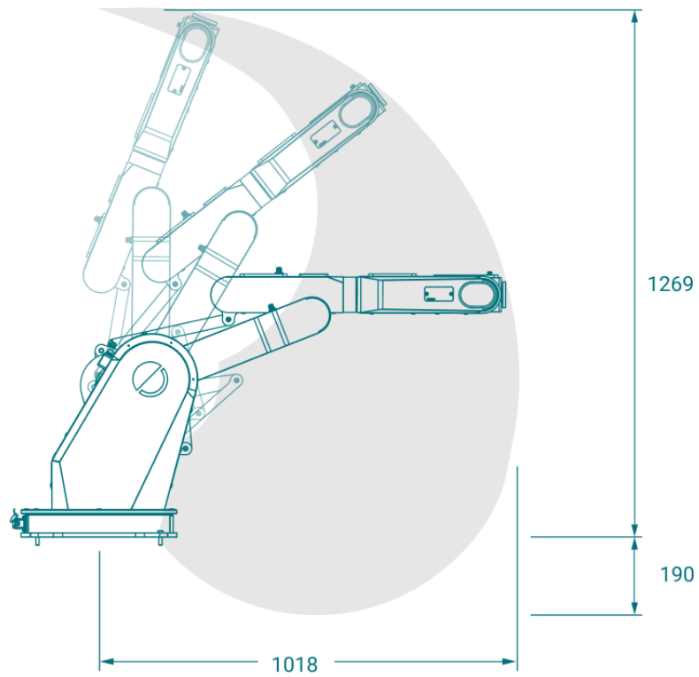
HORST1000 workspace: Lateral section
