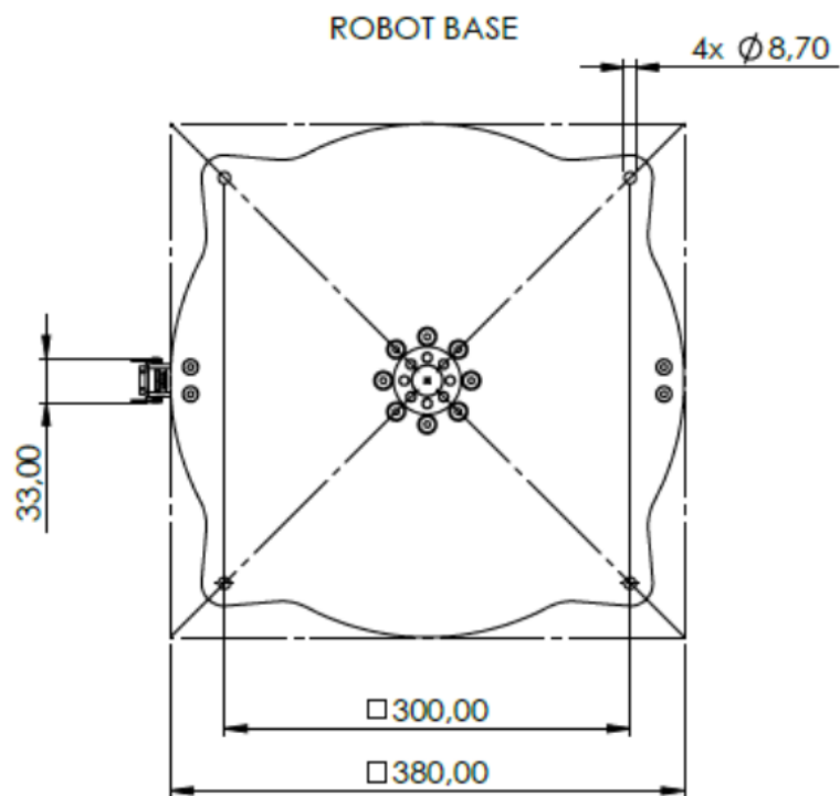
Dimensions of the installation area and base drilling pattern of HORST1000
