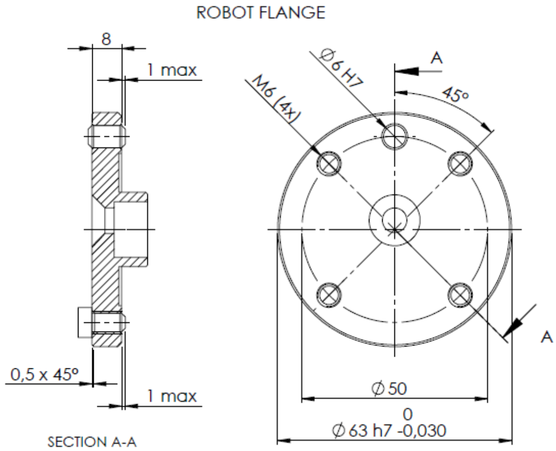
Robot flange of HORST1000
